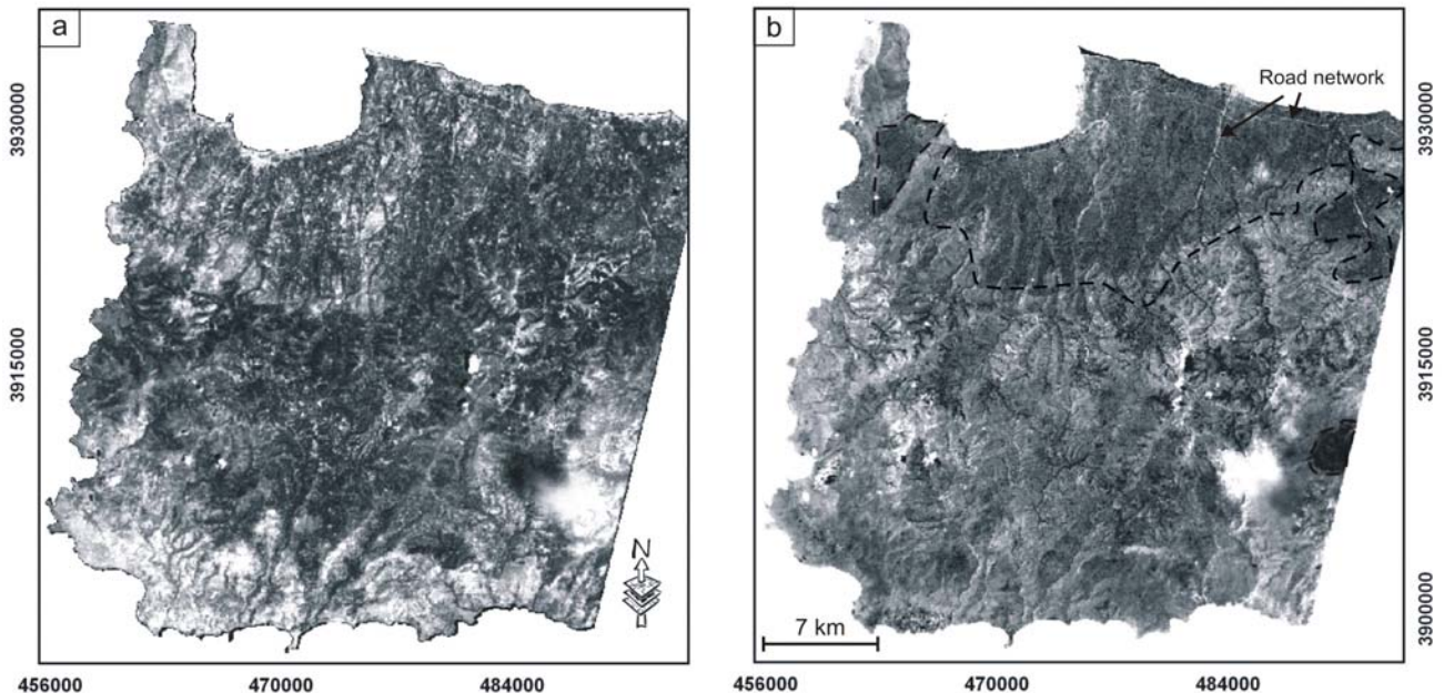
Figure 3: (a) The first Principal Component image for the VNIR and SWIR bands. In terms of analyzing the spectral properties of the surface materials, it is not easy to trace back the potential structural origin of lineaments on this PC1-VNIR&SWIR. This is because it is a weighted sum of the visible and SWIR spectral characteristics of the targets. (b) The second Principal Component image. The Neogene formations are illustrated in dark tones of grey and are clearly distinguished from the surrounding open area. The road network is also highlighted in light tones (black arrows to the NE part of the area).
