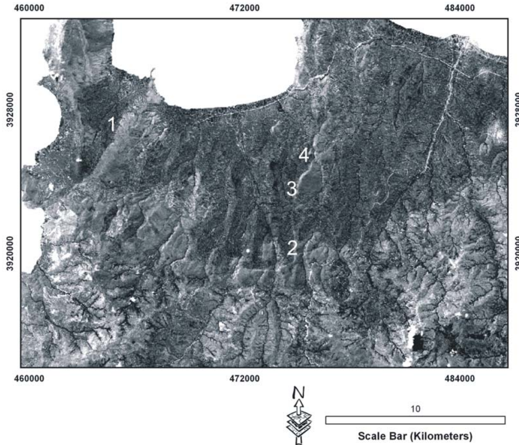
Figure 4: Image showing the second Principal Component image for the VNIR and SWIR bands (i.e., PC2-VNIR&SWIR). The Neogene sediments are characterized by relatively dark brightness values. Tectonic contacts between geological formations were established at locations 1 - 4 because of their distinct linear shape and tonal contrast with the surrounding area.
