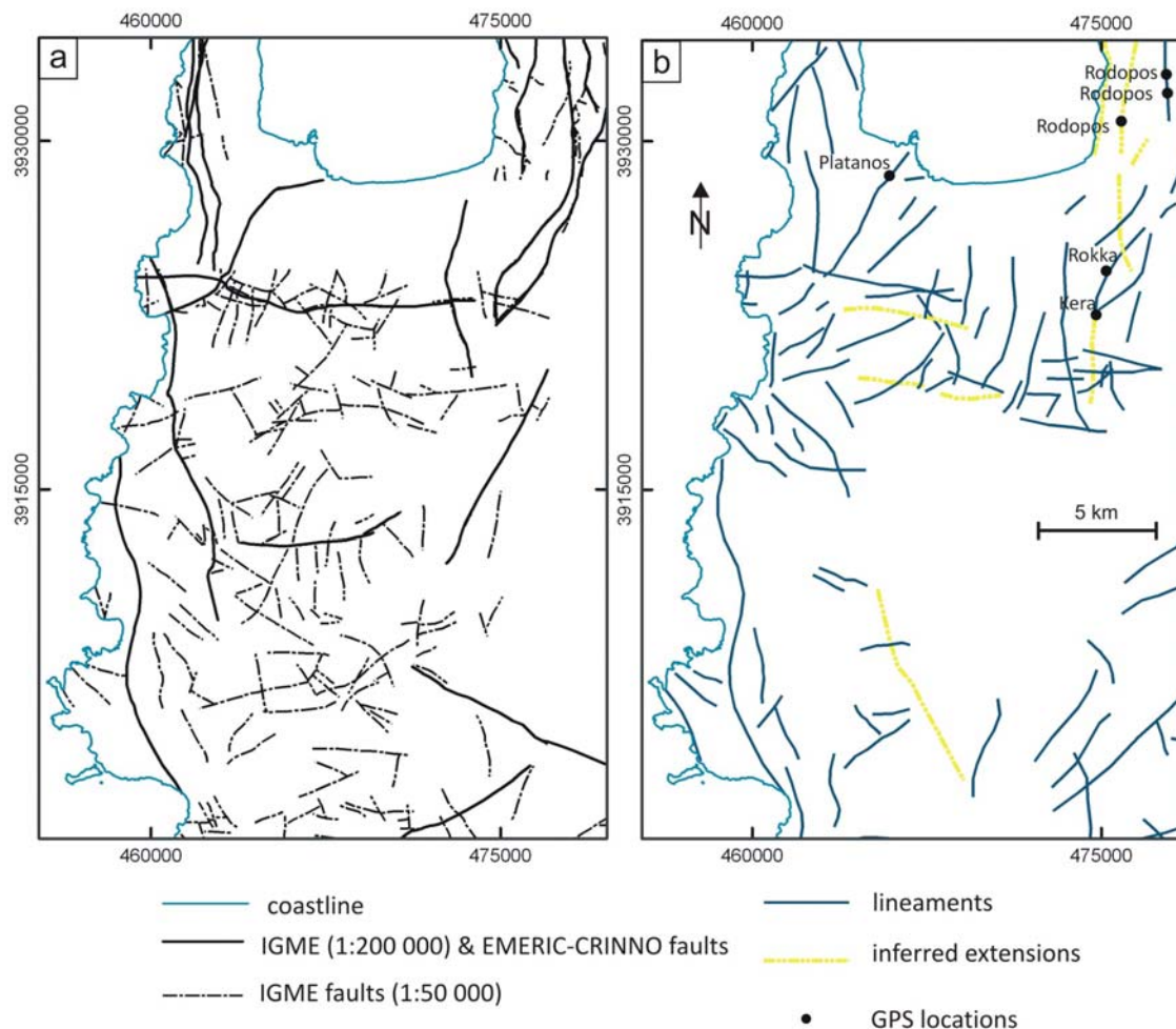
Figure 9: (a) Map of previously verified faults by IGME and EMERIC-CRINNO geological surveys. (b) Map showing the lineaments identified in the present work that might be attributed to failure of the crust. Limited fieldwork locations are also depicted. Especially in the case of macro-lineaments (>8 km) there is a good agreement between the two maps.
