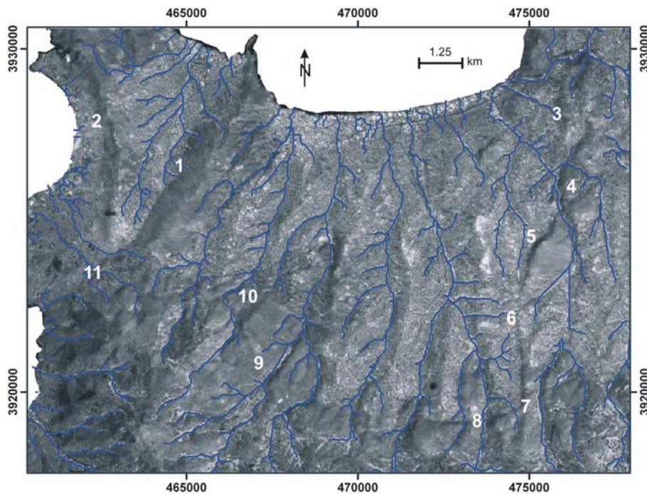
Figure 6: Overlay of the PC1-TIR component image and the near infrared-red image (ASTER Band 3N). Increased soil moisture appears in relatively dark brightness values. The solid blue lines represent the drainage lines digitized from the topographical maps of the area. Lineaments at locations No.1-11 have been evaluated as potential faults that control the drainage system of the area.
