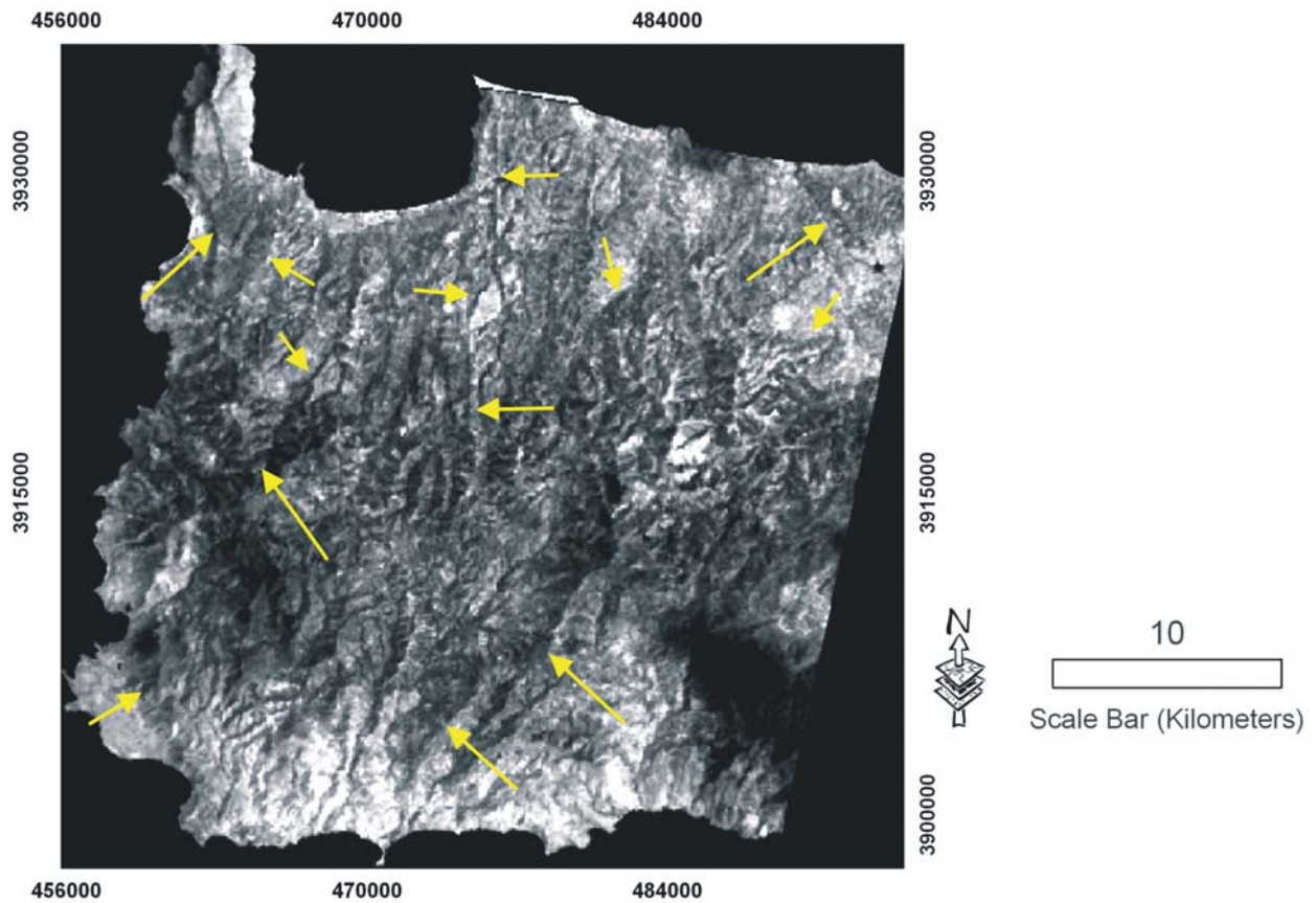
Figure 5: The PC1-TIR image showing linear features of low radiant temperature (dark brightness values). Despite the low spatial resolution, this particular image demonstrates numerous lineaments possibly related to increased soil moisture (yellow arrows).
