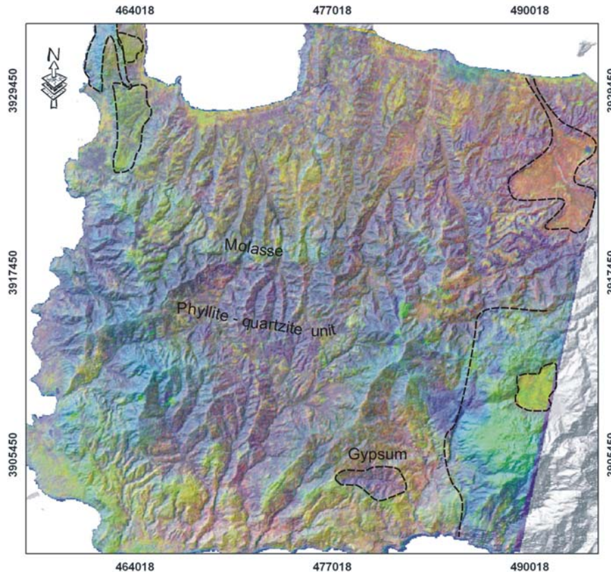
Figure 8: The three-band False Colour Composite image superimposed over the shaded relief of the area. Here colours are represented as PC1-TIR=Red, PC1 – VNIR & SWIR=Green and PC2 – VNIR & SWIR=Blue. The spectral information initially encompassed in the 14 original ASTER bands is compressed in a single RGB composite. Despite the fact that PC images used to form RGB composites are not easy to interpret, several geological formations are well delineated in this product.
