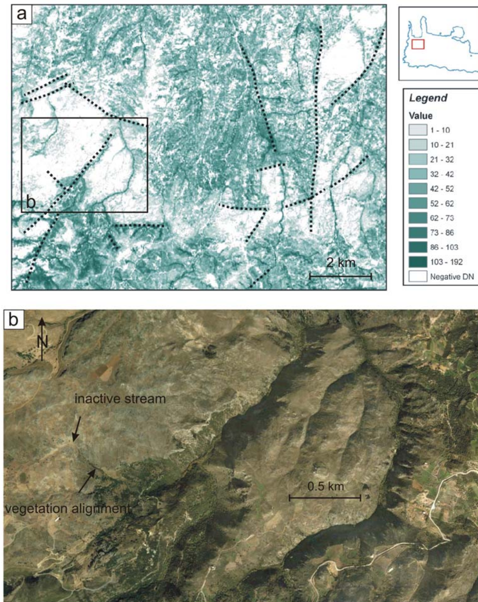
Figure 7: (a) Part of the segmented vegetation index image. The dotted lines refer to vegetation that is mainly but not exclusively developed along rivers. The higher values (for example the last two classes) represent very green areas (i.e., healthy vegetation retaining relatively high moisture content). (b) Google Earth image, illustrating a typical example of vegetation growth along a fault zone. The stream course seems to be also controlled by the fault.
