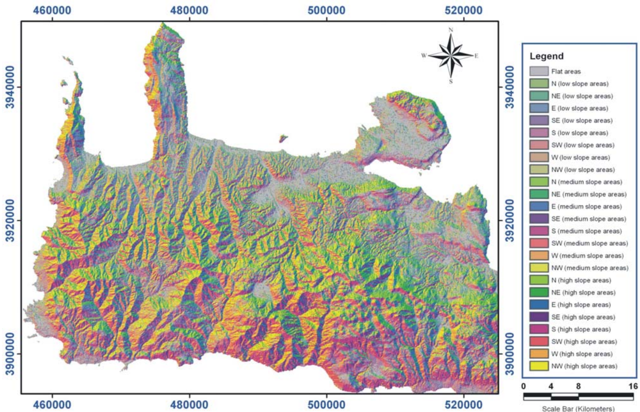
Figure 2: The aspect-slope map of the area. Flat areas are depicted in grey. The rest of the area is divided into 24 classes grouped in three main categories: 1) Low slope areas; 2) medium slope areas, and 3) high slope areas. Each of these categories is divided in eight different aspects (N, NE, E, SE, S, SW, W, NW). The steeper the slope (high slope areas in the legend) the brighter it appears.
