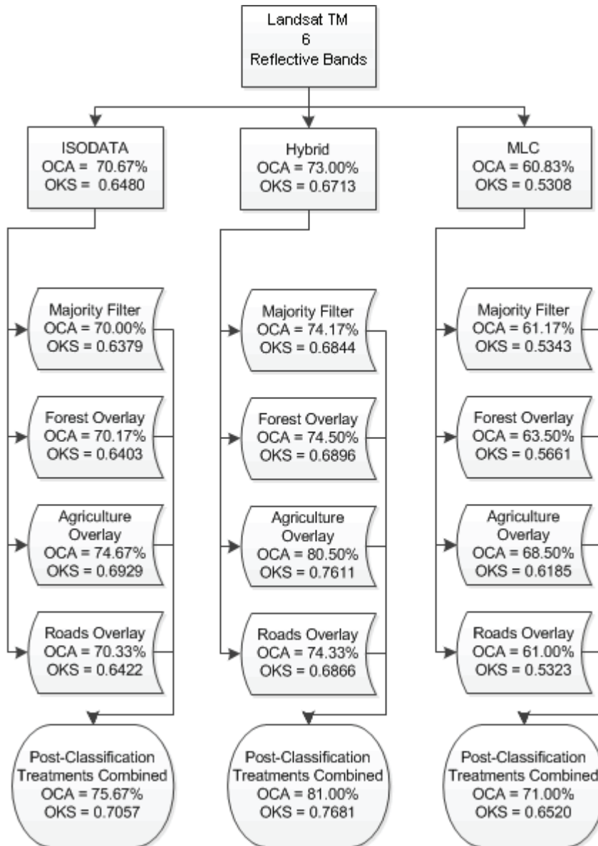
Figure 6: Accuracies obtained for Landsat TM reflective bands products, including the separate contribution of each stage of the DSS by itself. Accuracy measures used are the Overall Classification Accuracy (OCA) and the Overall Kappa Statistic (OKS).
