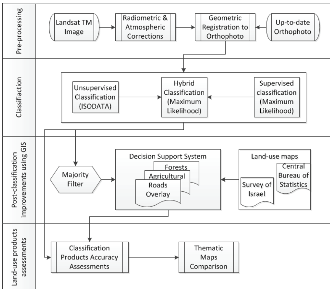
Figure 2: Research flowchart.
