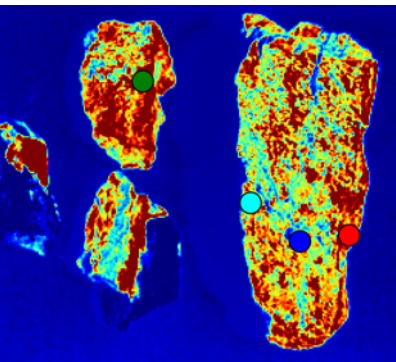
EnMAP
