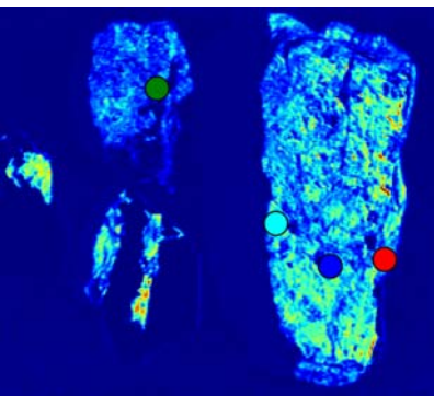
ASTER
