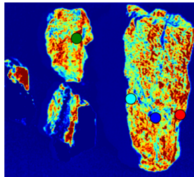
ALI
