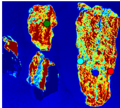
Sentinel-2
